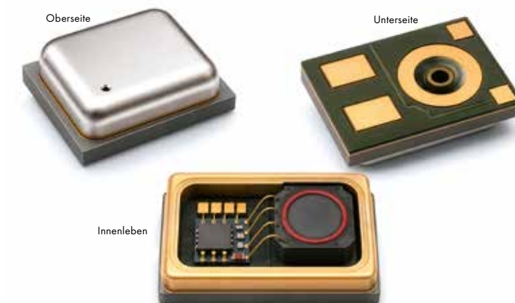
MEMS(Micro-Electronic-Mechanical-System)-Mikrofon
